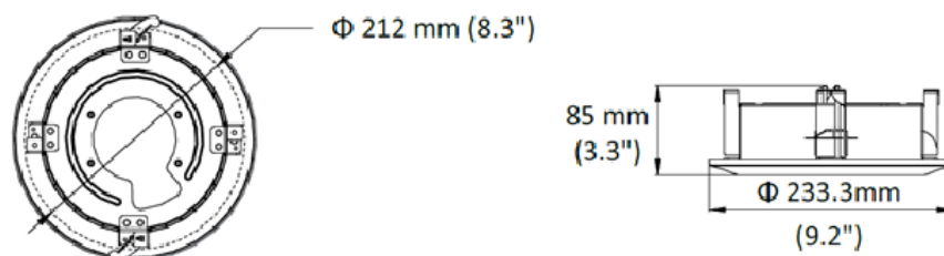
CM19 Dimension
