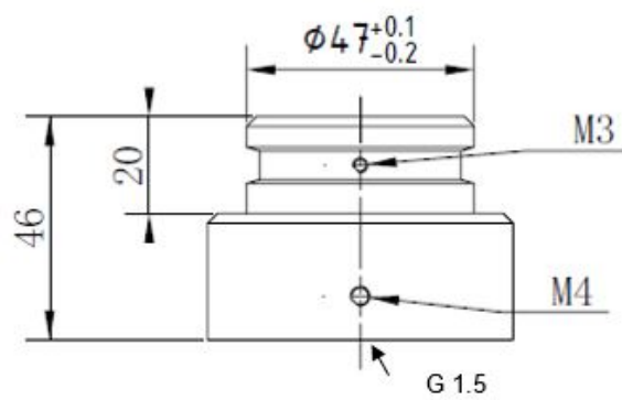
PTM02 Dimensions
