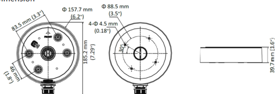
JB02 Dimension
