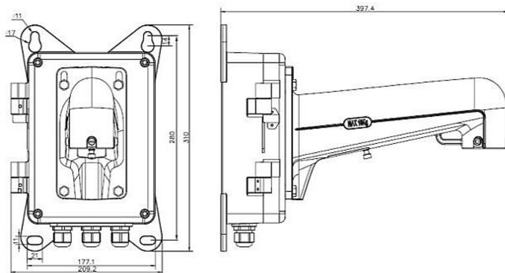
WM17 dimensions
