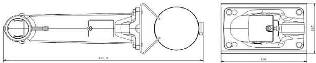
PM07 Dimensions
