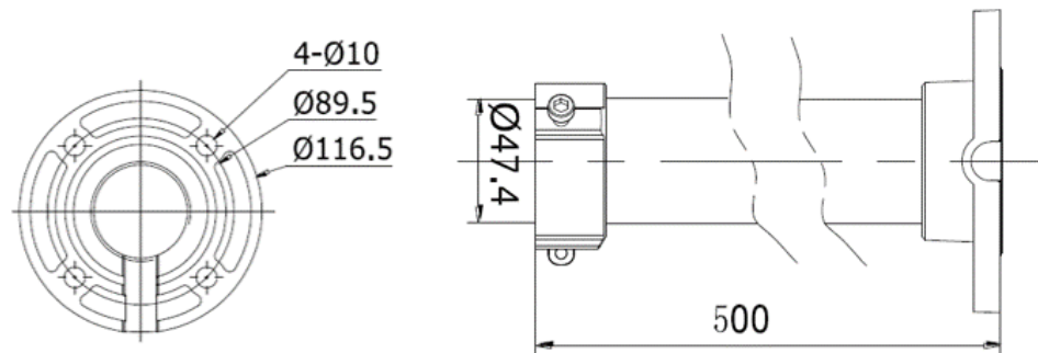
CM12 Dimension
