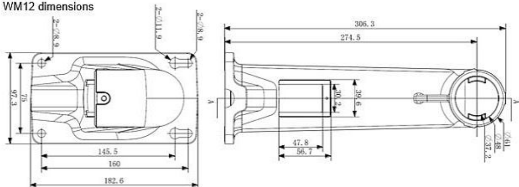
WM12B dimensions
