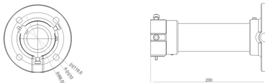
CM19 Dimension
