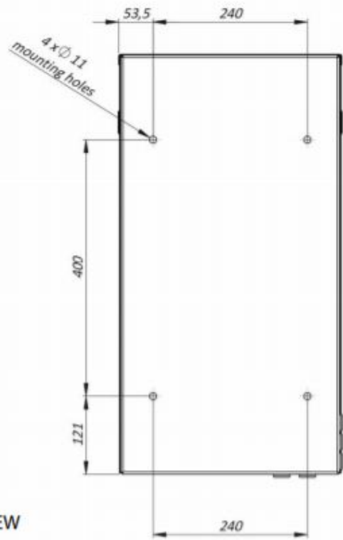
MOUNTING PATTERN
