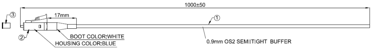
LC/UPC SM CONNECTOR
