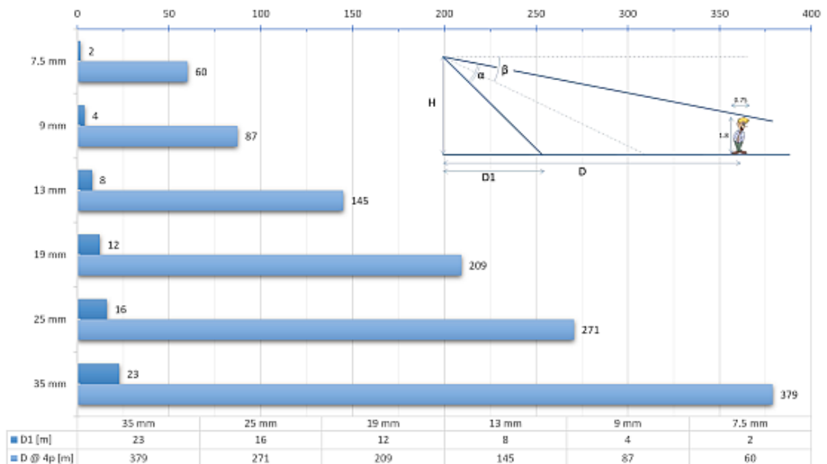
PID detection with 640x512 module - 6m high pole
